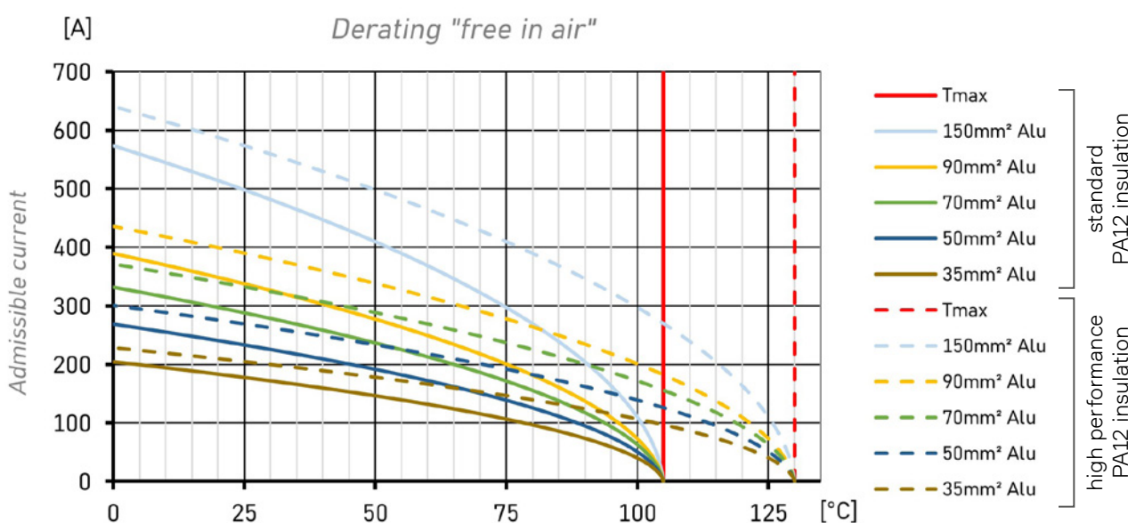
Figure 8 Derating curves for aluminium with standard PA12 insulation and high performance PA12 insulation
