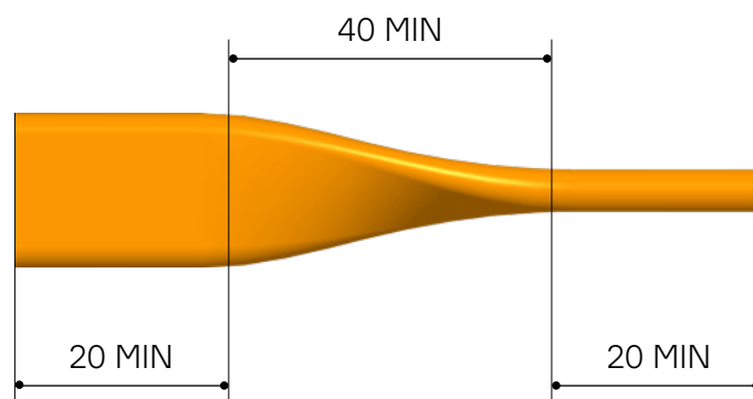
Figure 6 Minimum distances for twisting
