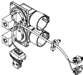
Fig. 1 - View of the angled connector - 2 connector variants
