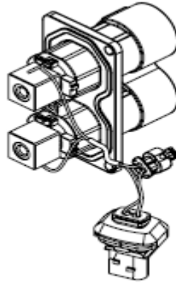
Fig. 2 - View of the straight connector - 2 connector variants
