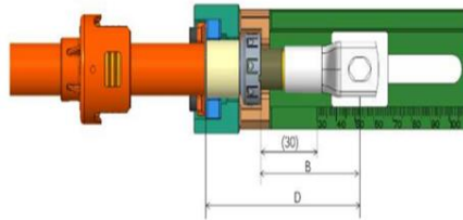
Fig. 1 - View of the bundle before the process of instaling and shrinking the HD1400 50mm 2 , 95mm 2 , 120mm 2 , 150mm 2
