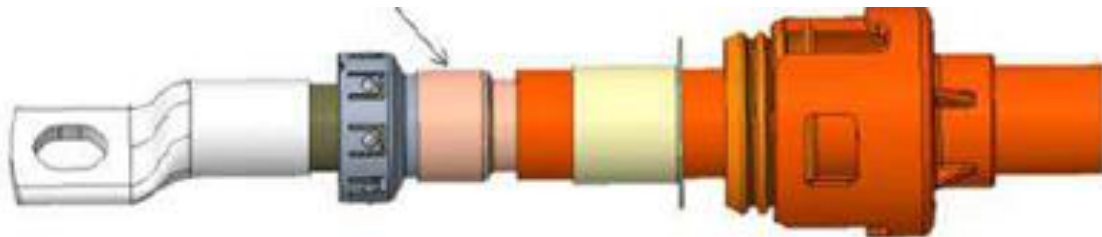
Fig. 3 – Preview of the cable before the ferrule assembly process – IPT HD connector – 50mm 2 , 70mm 2 , 95mm 2
