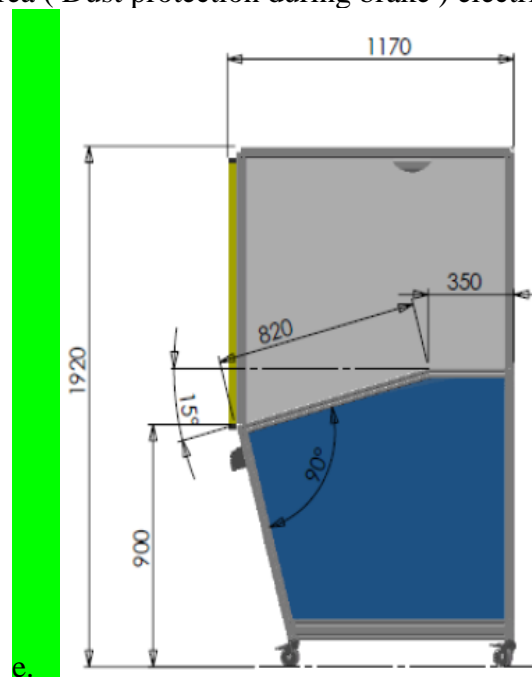
Fig. 1 – Graphical representation of the required dimensionality of the testing table
